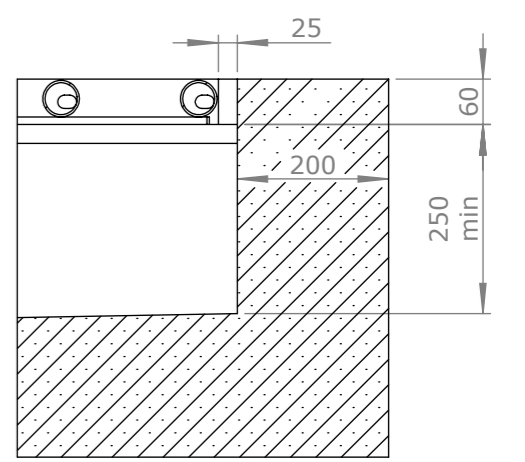
DETAIL F SCALE 1 : 10
