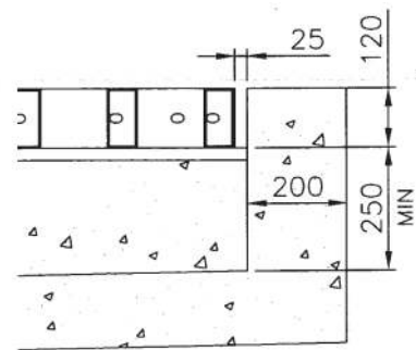
DETAIL - F
